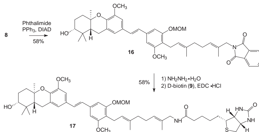
Scheme 3. Preparation of amide 17.
