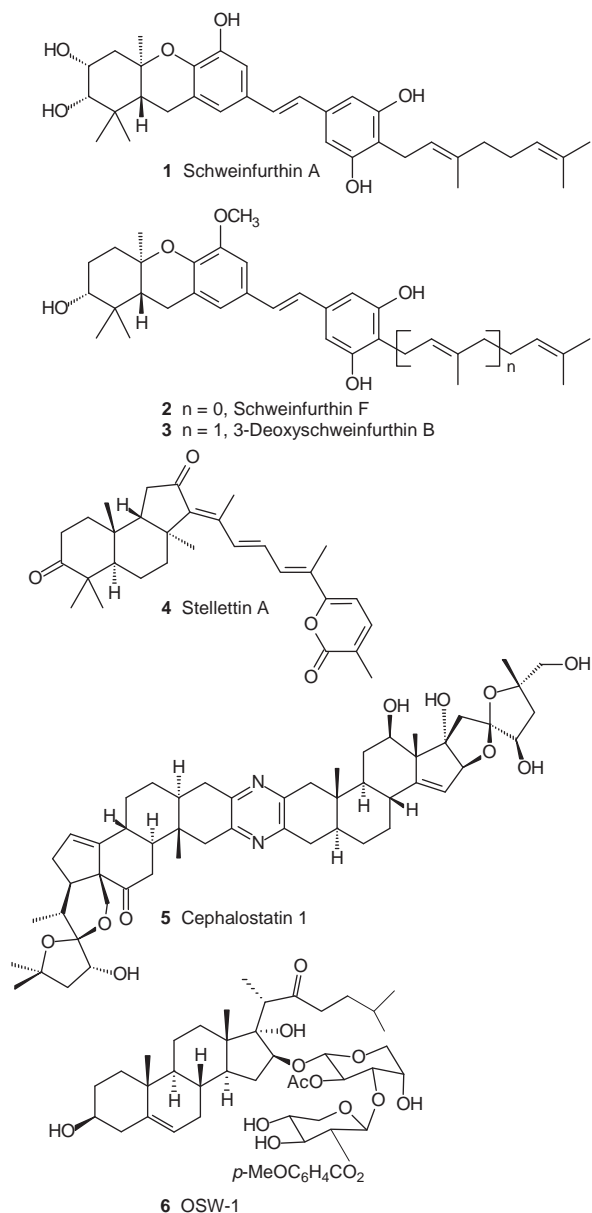
Figure 1. Some schweinfurthins ( 1–3 ), stelletin A ( 4 ), cephalostatin 1 ( 5 ), and OSW-1 ( 6 ).
