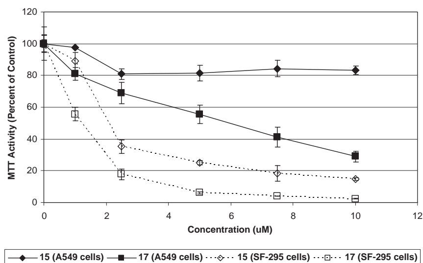
Figure 2. Concentration–response curves of compounds 15 and 17 in SF-295 and A549 cells. Values shown are the mean of quadruplicate treatments \pm the standard deviation.
